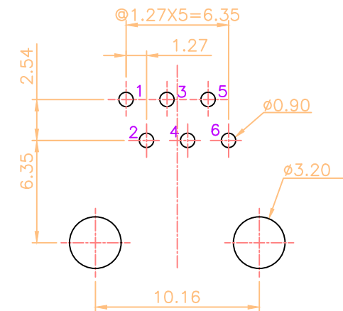
PC Board Layout Component Side Shown PC Board Thickness=1.6mm Tolerance±0.05
